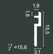
C395 STEPS 200 x 15,5 x 3,1 cm Purotouch® Designed by Orio Tonini
