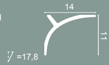
C991 200 x 11 x 14 cm Purotouch ® Designed by Ulf Moritz
