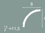
C240 | C240F 200 x 8 x 8 cm Purotouch ®
