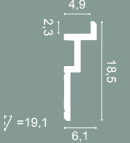
C396 STEPS 200 x 6,1 x 18,5 cm Purotouch® Designed by Orio Tonini
