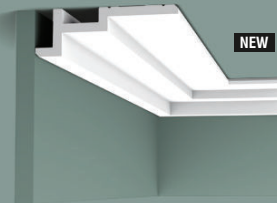
C396 STEPS 200 x 6,1 x 18,5 cm Purotouch® Designed by Orio Tonini
